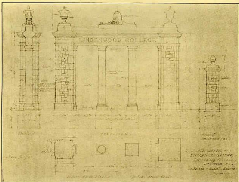
ENTRANCE TO BUTLER WAY Architect's Working Drawing
